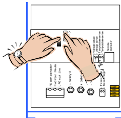
Justering, maksimal Bulk strøm
